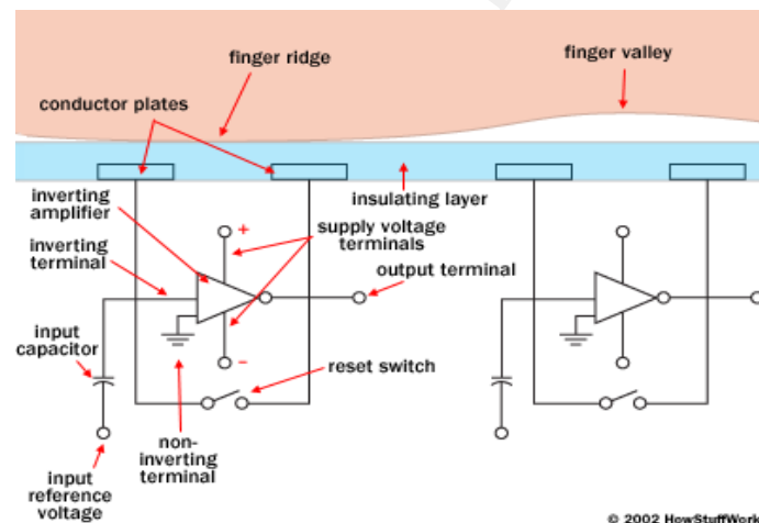
Figure 4 Capacitive Scanning
