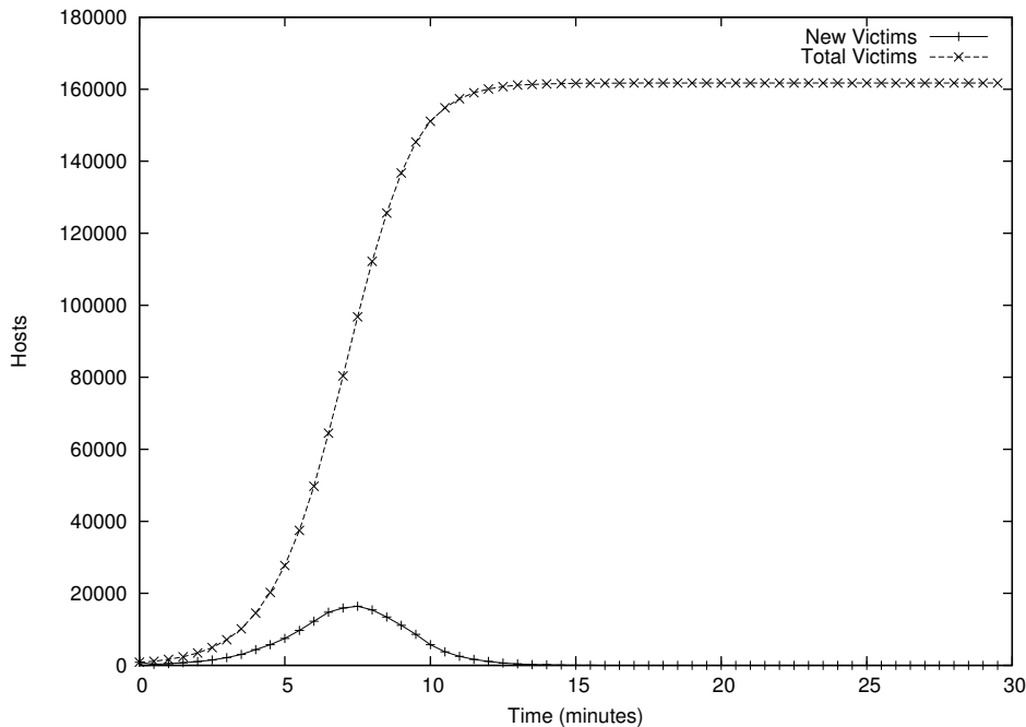
Figure 12: Pre-scanning with pre-infection
