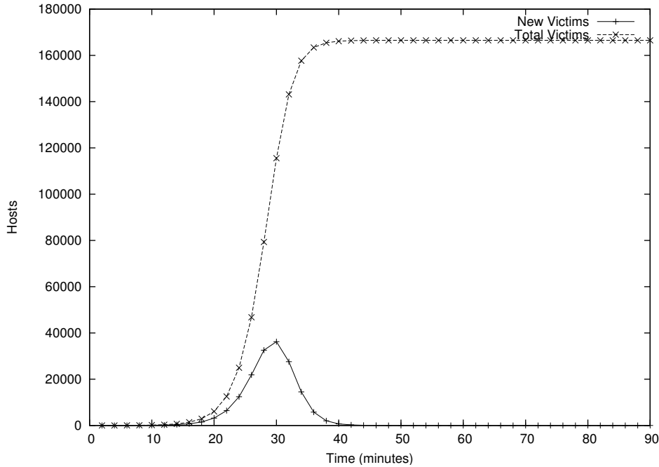
Figure 5: Multi-threading, parallel worm with random propagation
