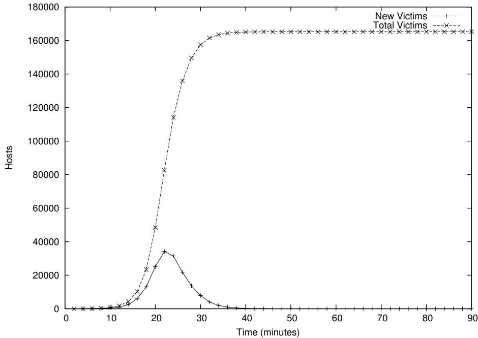
Figure 7: Local preference with multi-threading and short timeouts
