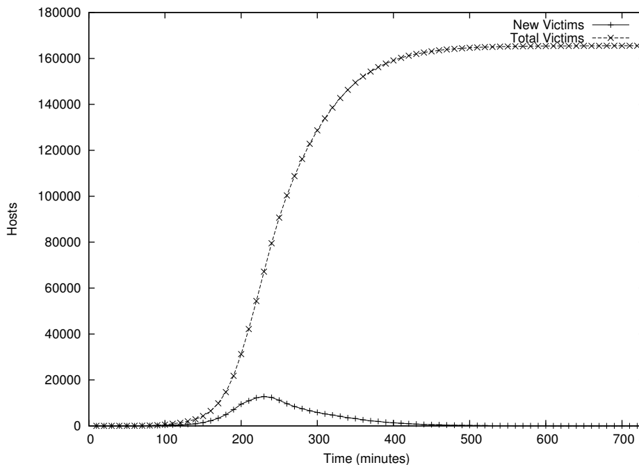
Figure 6: Local preference propagation
