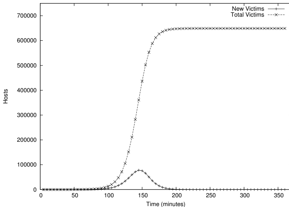
Figure 9: Worm with a higher vulnerable population
