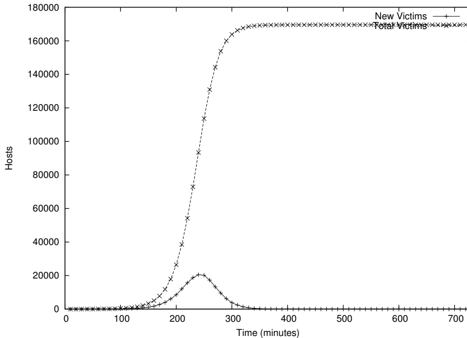
Figure 3: Random dataset and propagation with reduced timeouts
