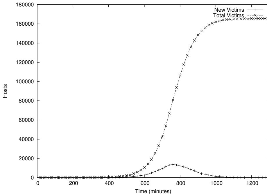
Figure 8: Sequential-scanning worm
