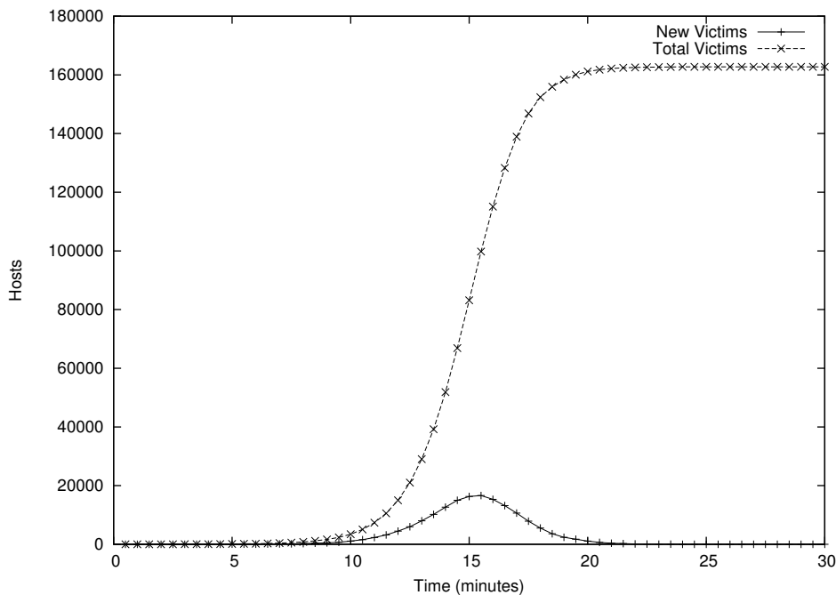
Figure 11: Pre-scanning /26 networks
