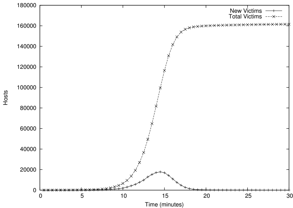
Figure 13: Adaptive behaviour of a scanning worm
