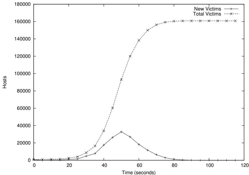
Figure 16: Advanced Multi-Threading Worm
