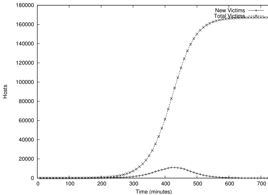
Figure 1: Initial, random dataset with random propagation algorithm
