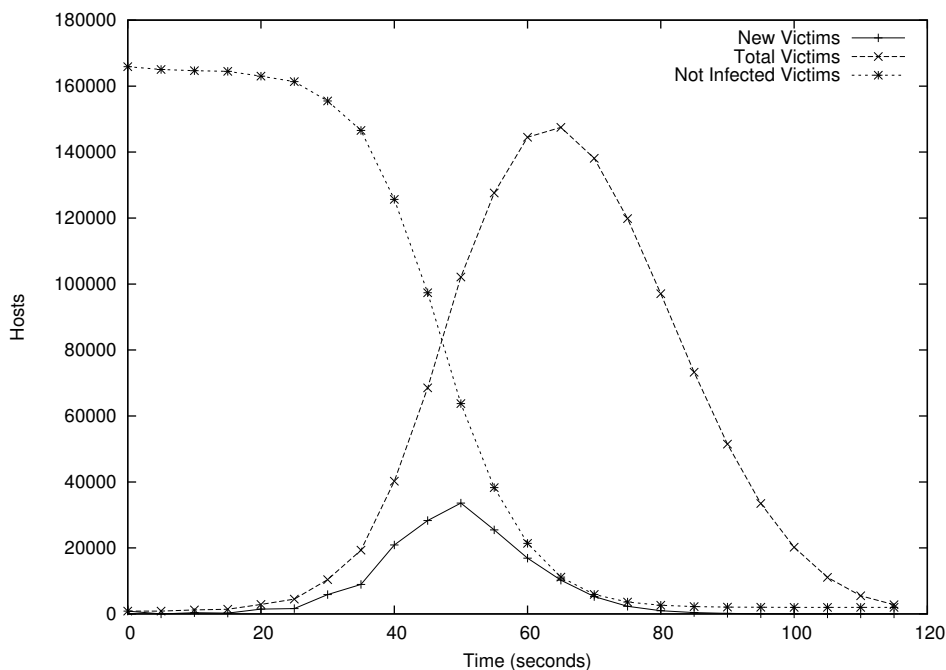
Figure 18: Advanced Worm with destructive payload
