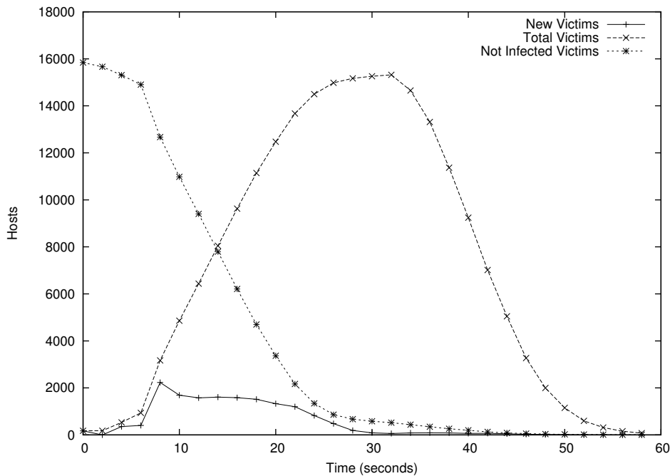
Figure 19: Local Network Destruction
