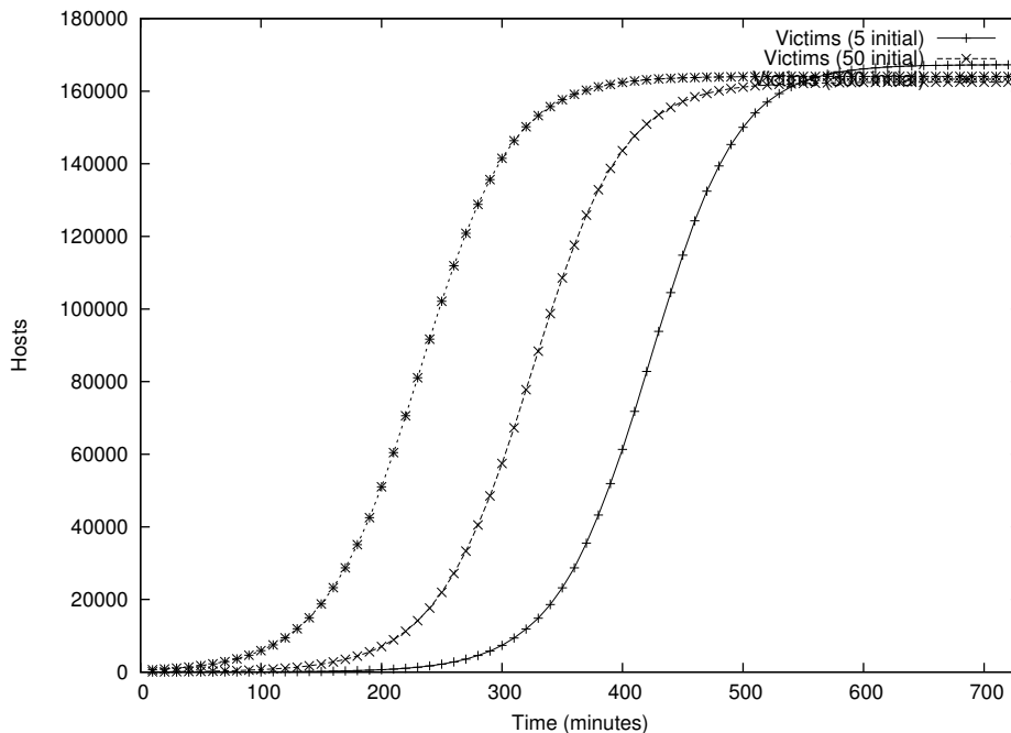
Figure 2: Random dataset and propagation with various numbers of pre-infected systems
