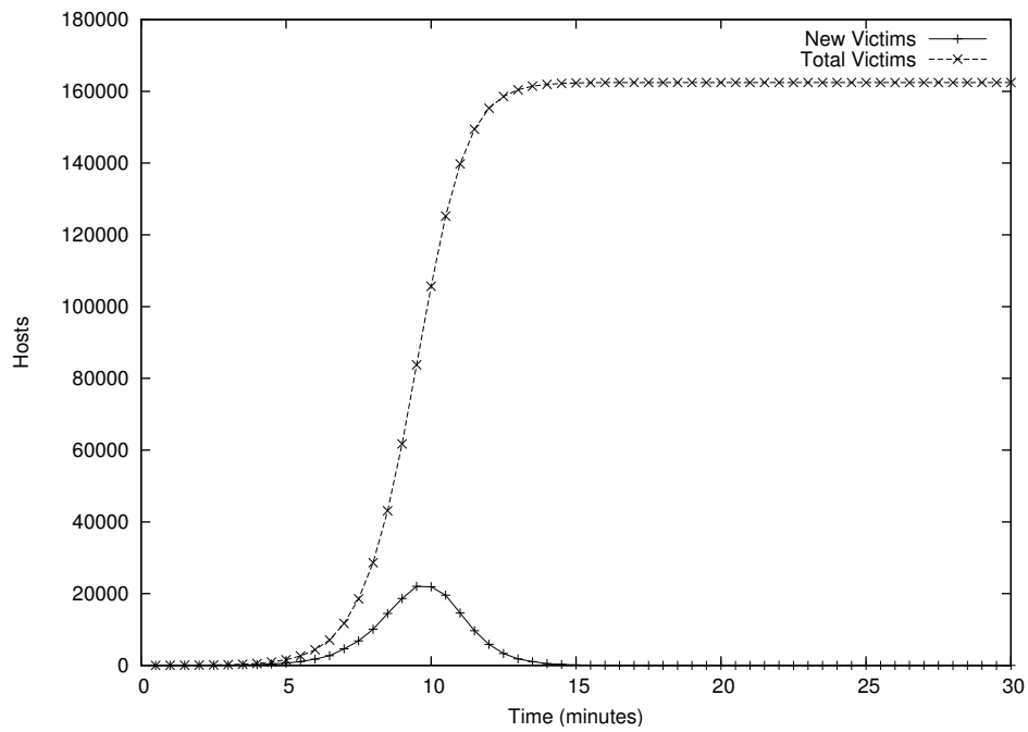
Figure 14: Pre-scanning worm with do-not-enter zones
