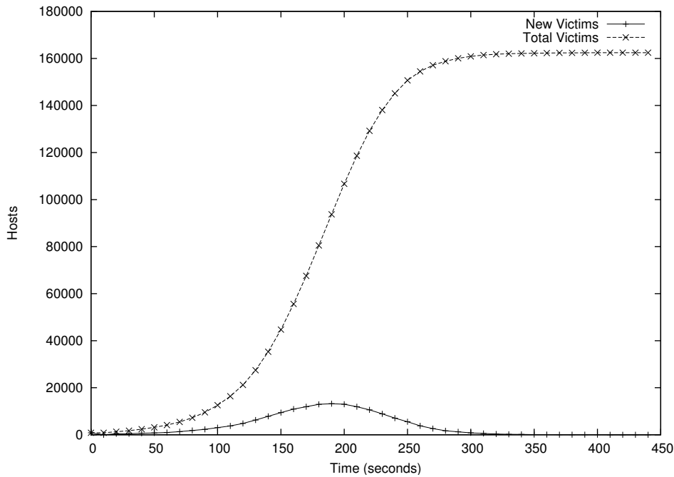
Figure 15: Advanced Worm
